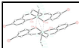
Fig. 2. A pair of inversion-related molecules, showing the intermolecular weak interactions between Mn and O phenolate atoms. The 'A' molecule is related to the 'B' molecule by [A: (x, y, z) \rightarrow B: (2-x, 1-y, -z)].
